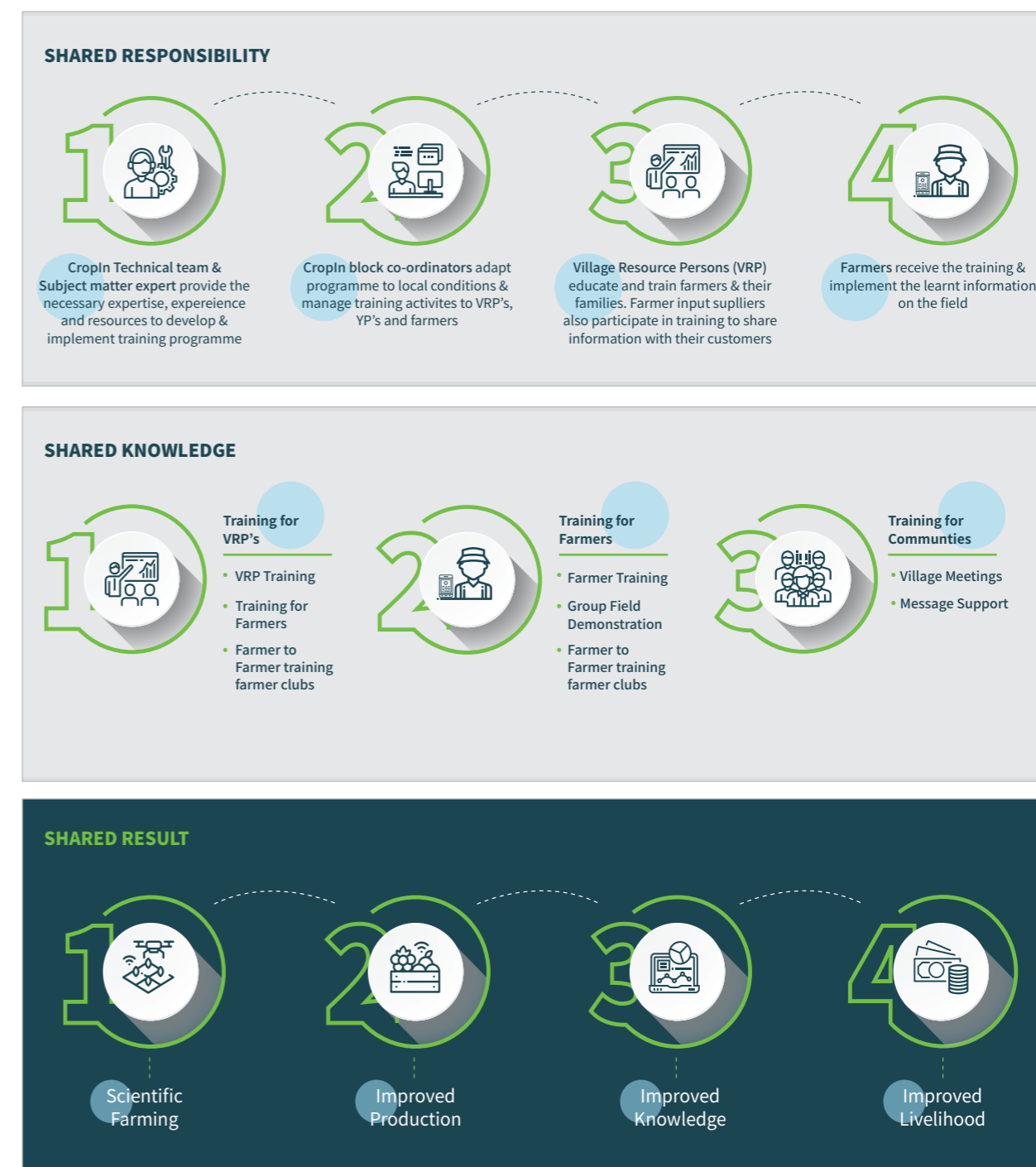
Image 3: Training Methodology
